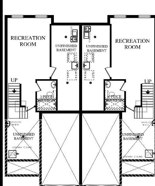
UNIT A 401 ELLESMER AVE. LOT 77 KINGS LANDING UNIT B 403 ELLESMER AVE. LOT 77 KINGS LANDING BASEMENT FLOOR PLAN
