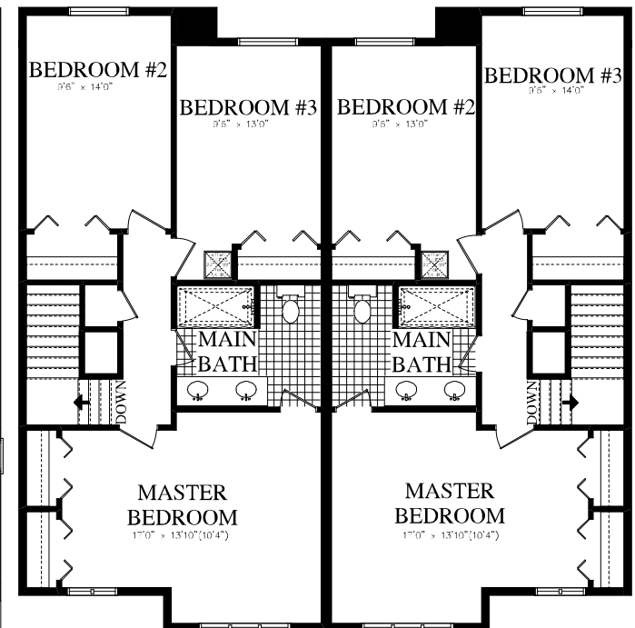
UNIT A 401 ELLESMER AVE. LOT 77 KINGS LANDING UNIT B 403 ELLESMER AVE. LOT 77 KINGS LANDING SECOND FLOOR PLAN
